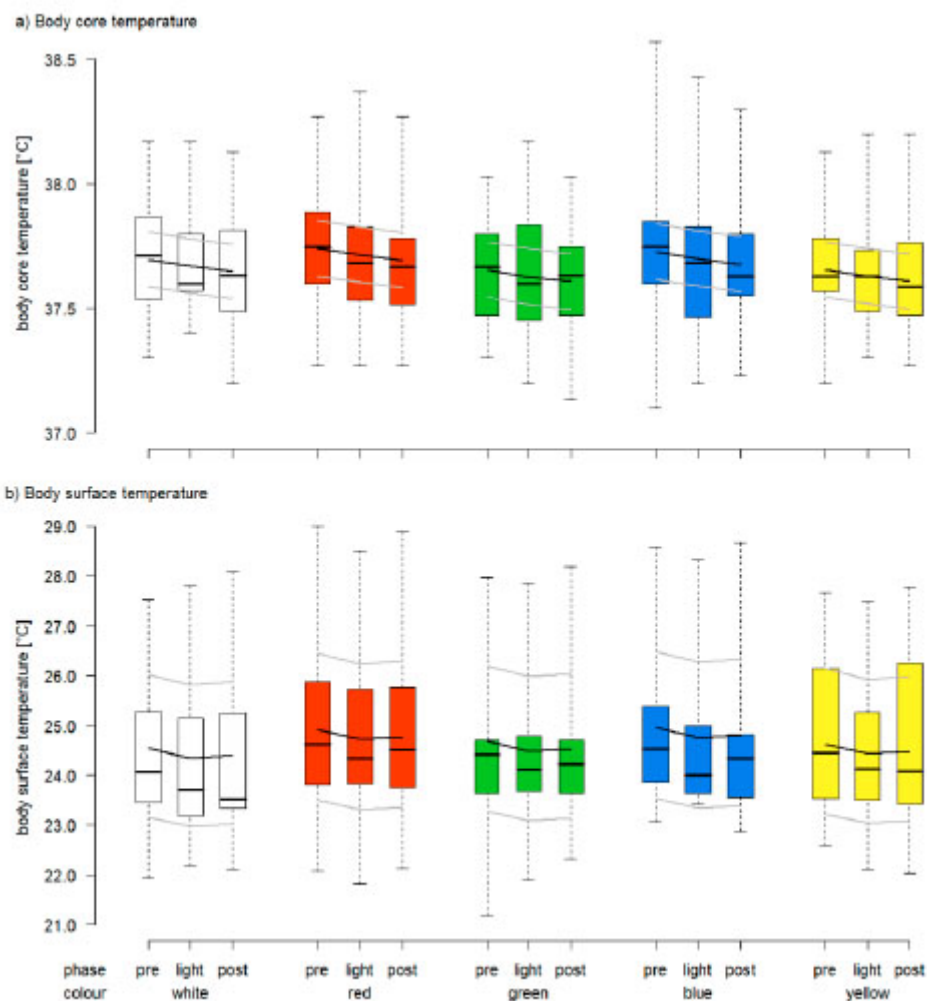
Fig. (7). a) Body core temperature [°C] and b) Body surface temperature [°C] in relation to colour and experimental phase (pre-, light-, post-phase) measured subsequent to the respective phase. Raw data are given as boxplots with medians, interquartile and absolute ranges, in addition to model predictions with estimated means (black lines) and 95% confidence intervals (grey lines).
