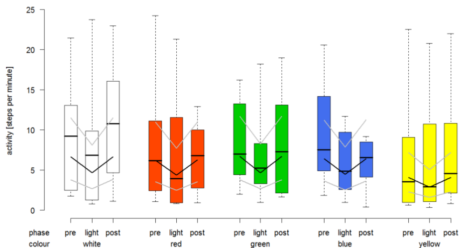
Fig. (4). Activity [steps per minute] in relation to colour and experimental phase (pre-, light-, post-phase). Raw data are given as boxplots with medians, interquartile and absolute ranges, in addition to model predictions with estimated means (black lines) and 95% confidence intervals (grey lines).
