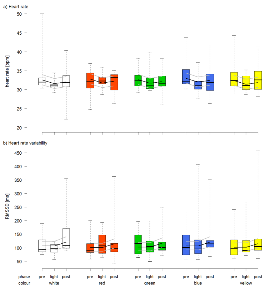
Fig. (6). a) Heart rate [beats per min] and b) Heart rate variability as RMSSD [ms] in relation to colour and experimental phase (pre-, light-, post-phase). Raw data are given as boxplots with medians, interquartile and absolute ranges, in addition to model predictions with estimated means (black lines) and 95% confidence intervals (grey lines).
